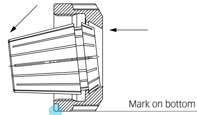
Disassembling
